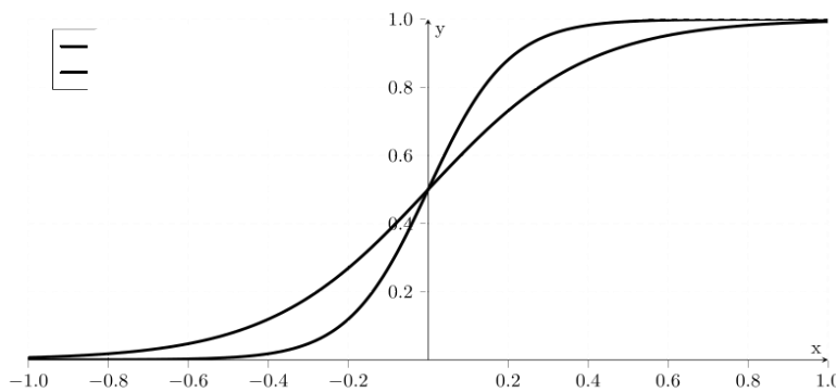
Figure 6 – Sigmoid function
