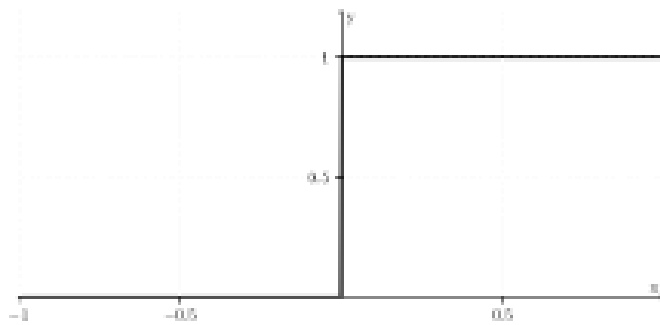
Figure 5 – Limit function
