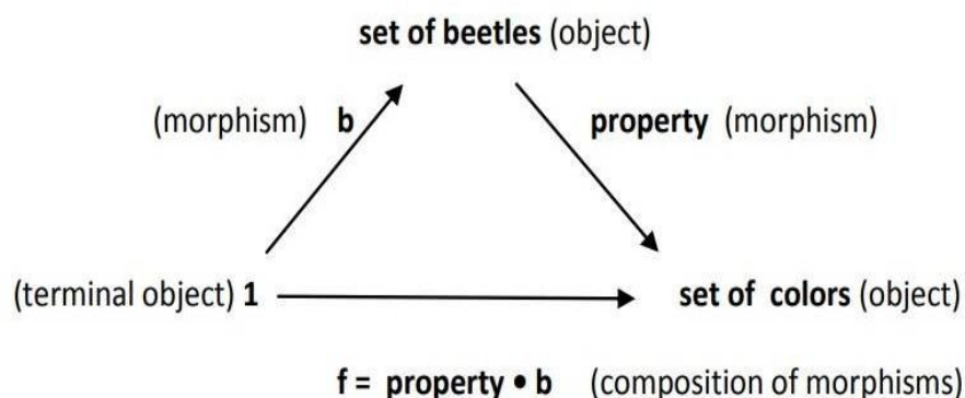
Figure 1 – Logical predicates
