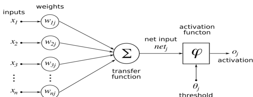
Figure 3 – Artificial neuron
