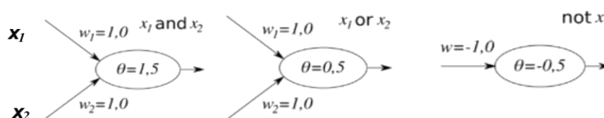
Figure 7 – Boolean functions
