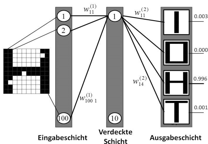
Figure 10 – Boolean computation
