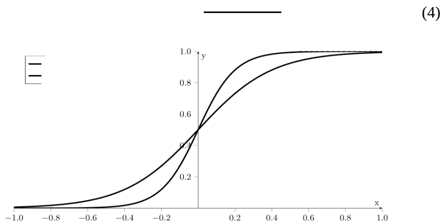
Figure 6 – Sigmoid function
